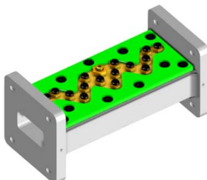
Waveguide Filter
